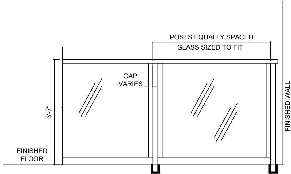
TYPICAL ELEVATION
