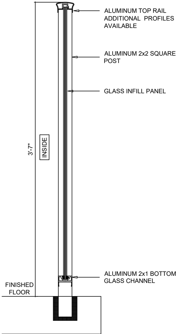
RAIL SECTION
