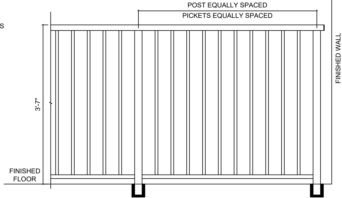
TYPICAL ELEVATION
